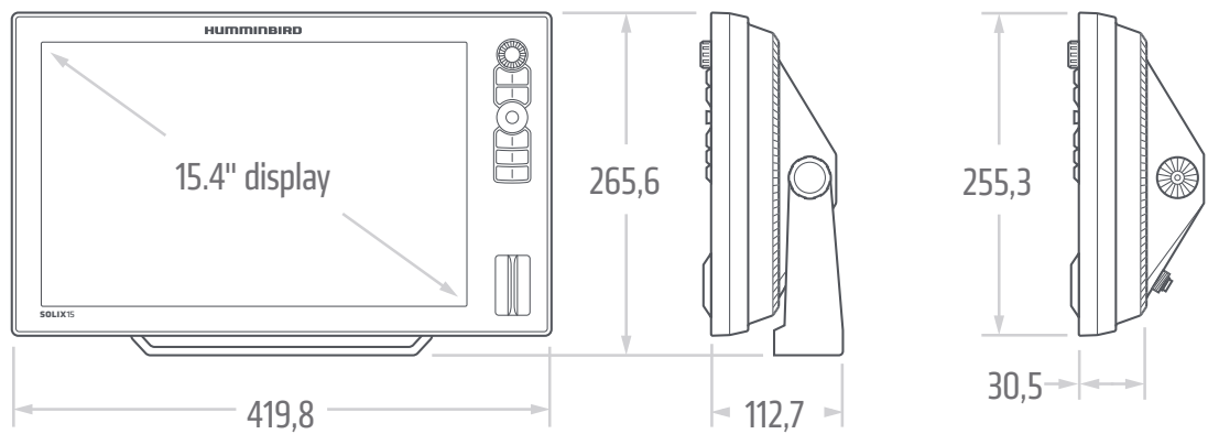
Gimbal Mount
