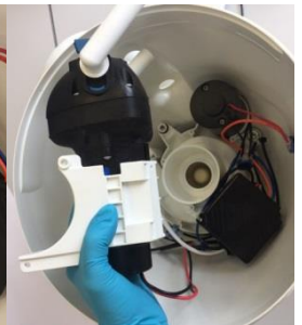
5. Remove pump
