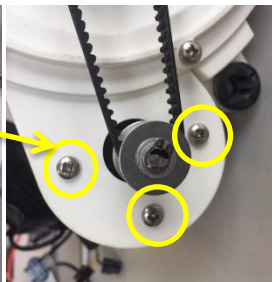
10. Remove screws
