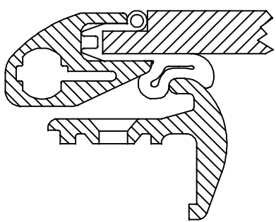
HATCH CROSS SECTION
