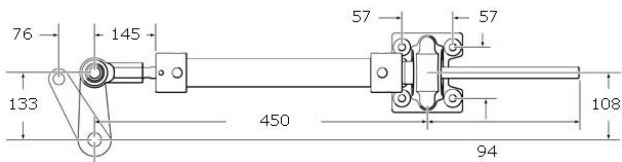
Attachment to tiller arm
