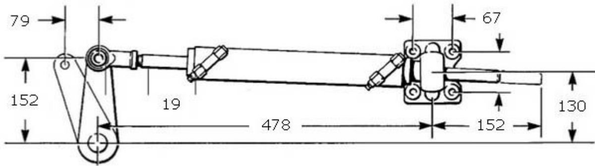
Attachment to tiller arm
