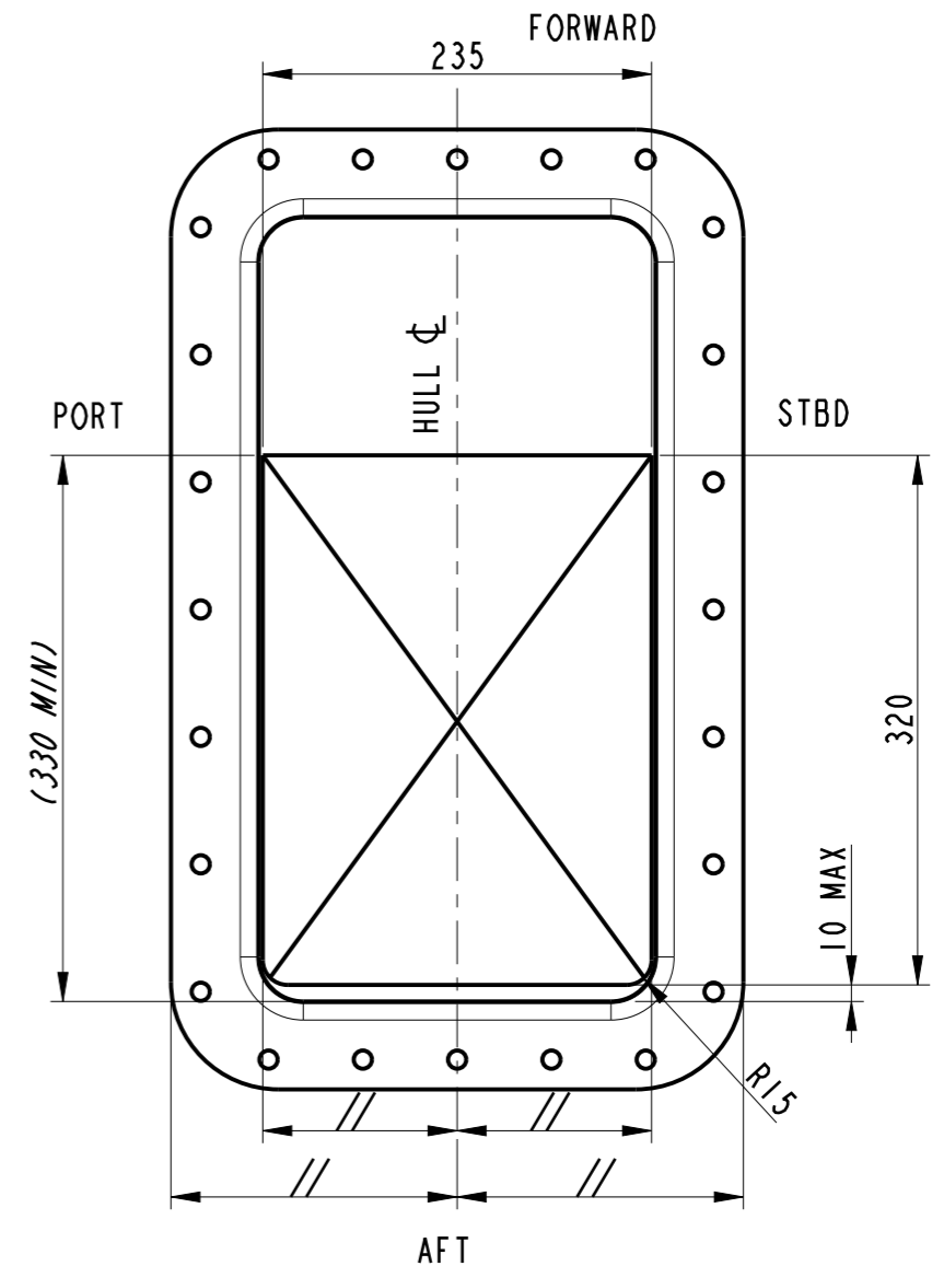
PLAN VIEW OF CUT-OUT VIEWED PARALLEL TO FLANGE SEALING FACE DIMENSION ARE MINIMUM REQUIRED SCALE 1:5 @ A3
