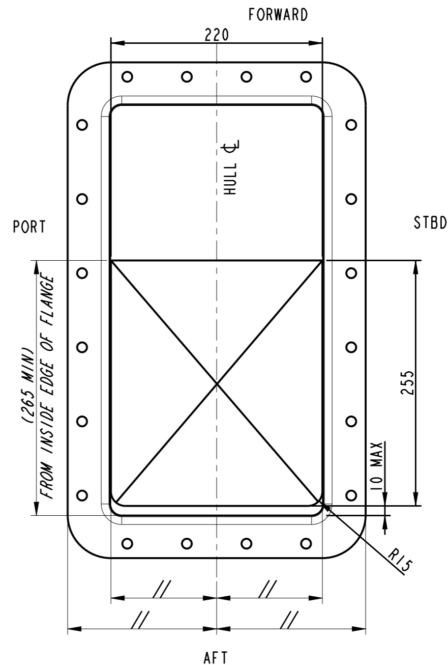
PLAN VIEW OF CUT-OUT VIEWED PARALLEL TO FLANGE SEALING FACE DIMENSION ARE MINIMUM REQUIRED SCALE 1:4 @ A3
