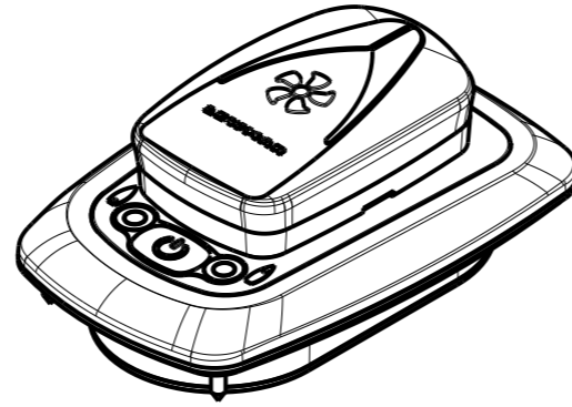
ISOMETRIC VIEW WITHOUT SUN COVER SCALE 1:2
